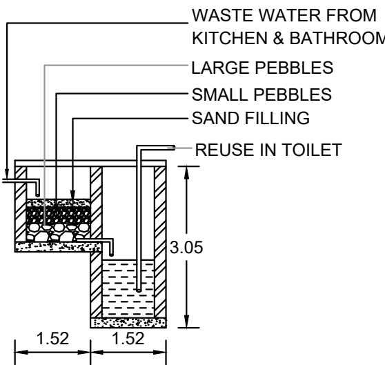
RECYCLING OF WASTEWATER FROM BATHROOM
