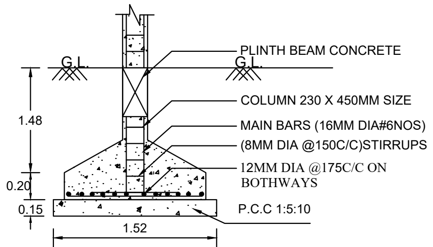
COLUMN FOOTING
