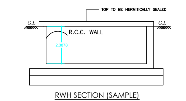
RWHS SECTION (SAMPLE)
