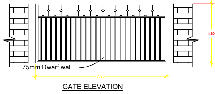
GATE ELEVATION
