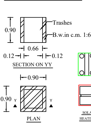
WASTE TRASH PIT
