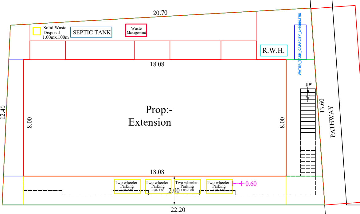
SITE PLAN
