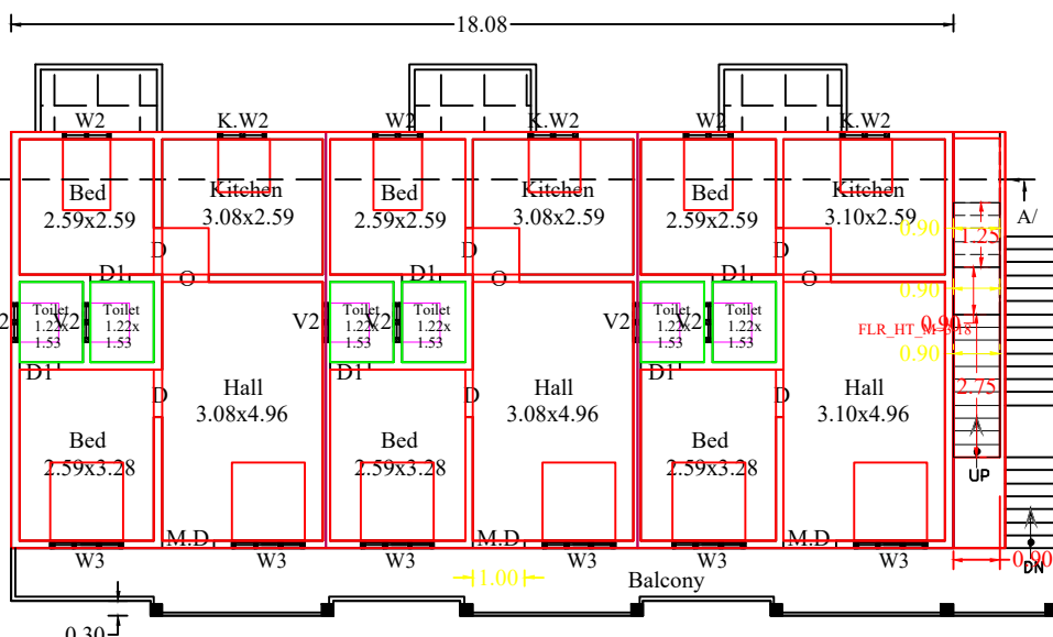
EXTENSION FIRST FLOOR PLAN
