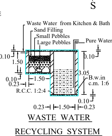
WASTE WATER RECYCLING SYSTEM
