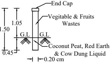
PIPE COMPOSTER
