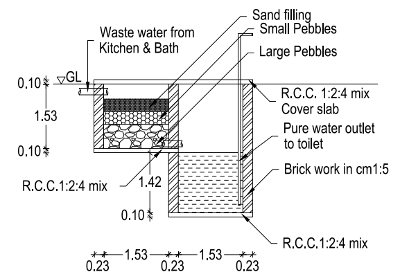
WASTE WATER RECYCLING SYSTEM HARVESTING PIT
