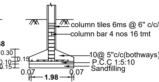
SECTION OF COLUMN
