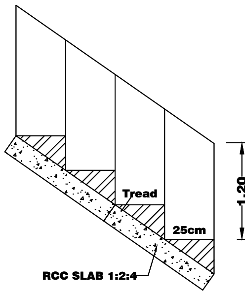
STAIR DETAILS
