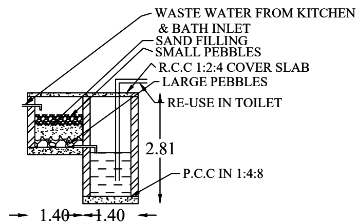
RECYCLING OF WASTE WATER KITCHEN & BATHROOM
