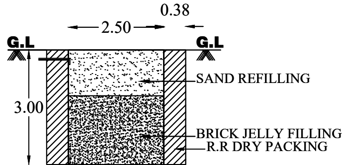
RAINWATER HARVESTING
