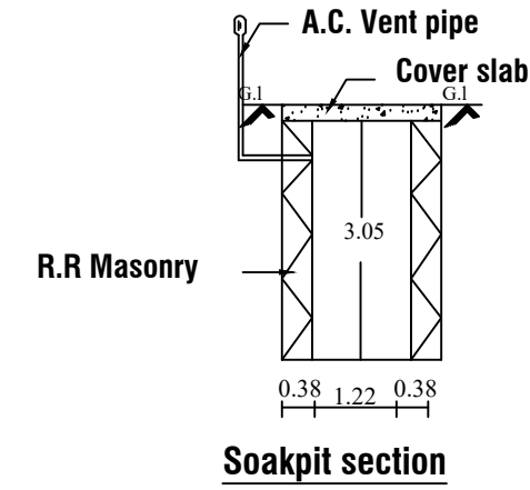
Soakpit section
