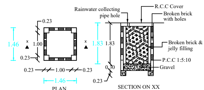
RWHTCAPACITY_L=6642LTRS
