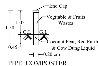
PIPE COMPOSTER
