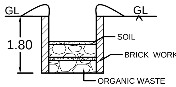
COMPOST PIT
