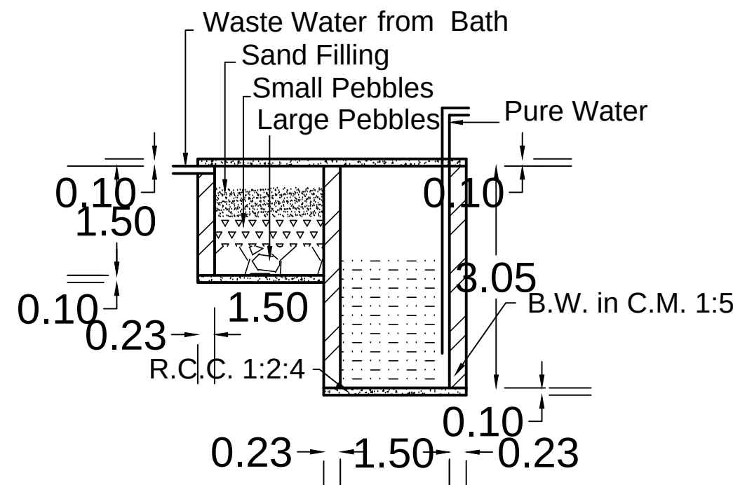
RECYCLING SYSTEM
