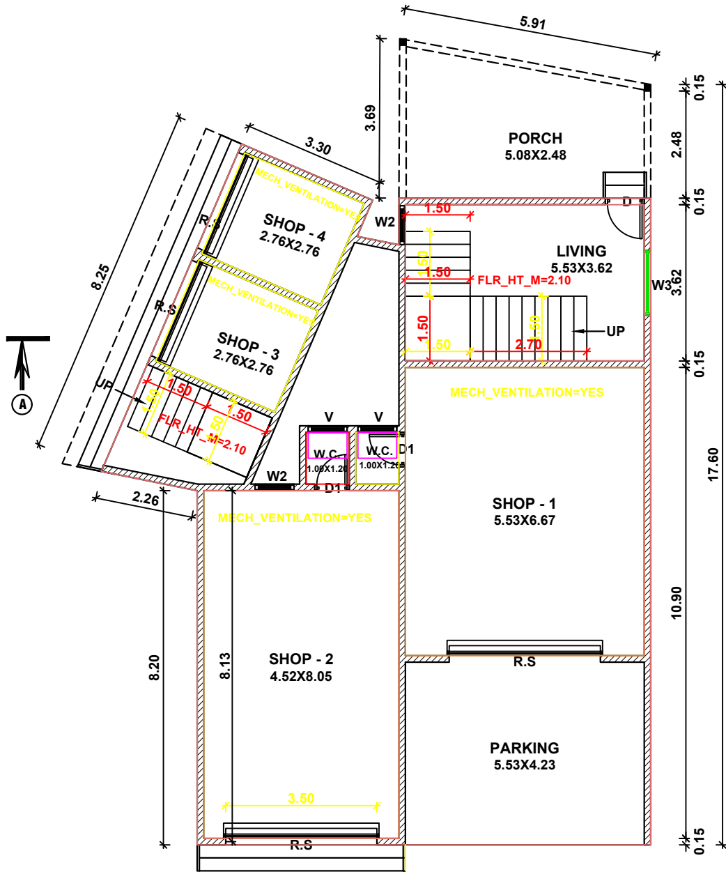
FLOOR PLAN
