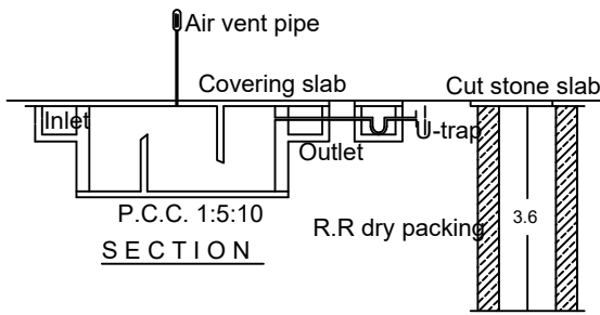
DETAILS OF RECYCLING OF WASTE WATER FROM KITCHEN & TOILET
