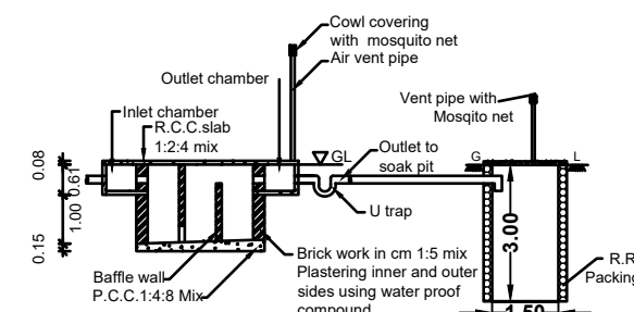
compound SECTION OF SEPTIC TANK & SOAK PIT
