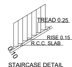
STAIRCASE DETAIL
