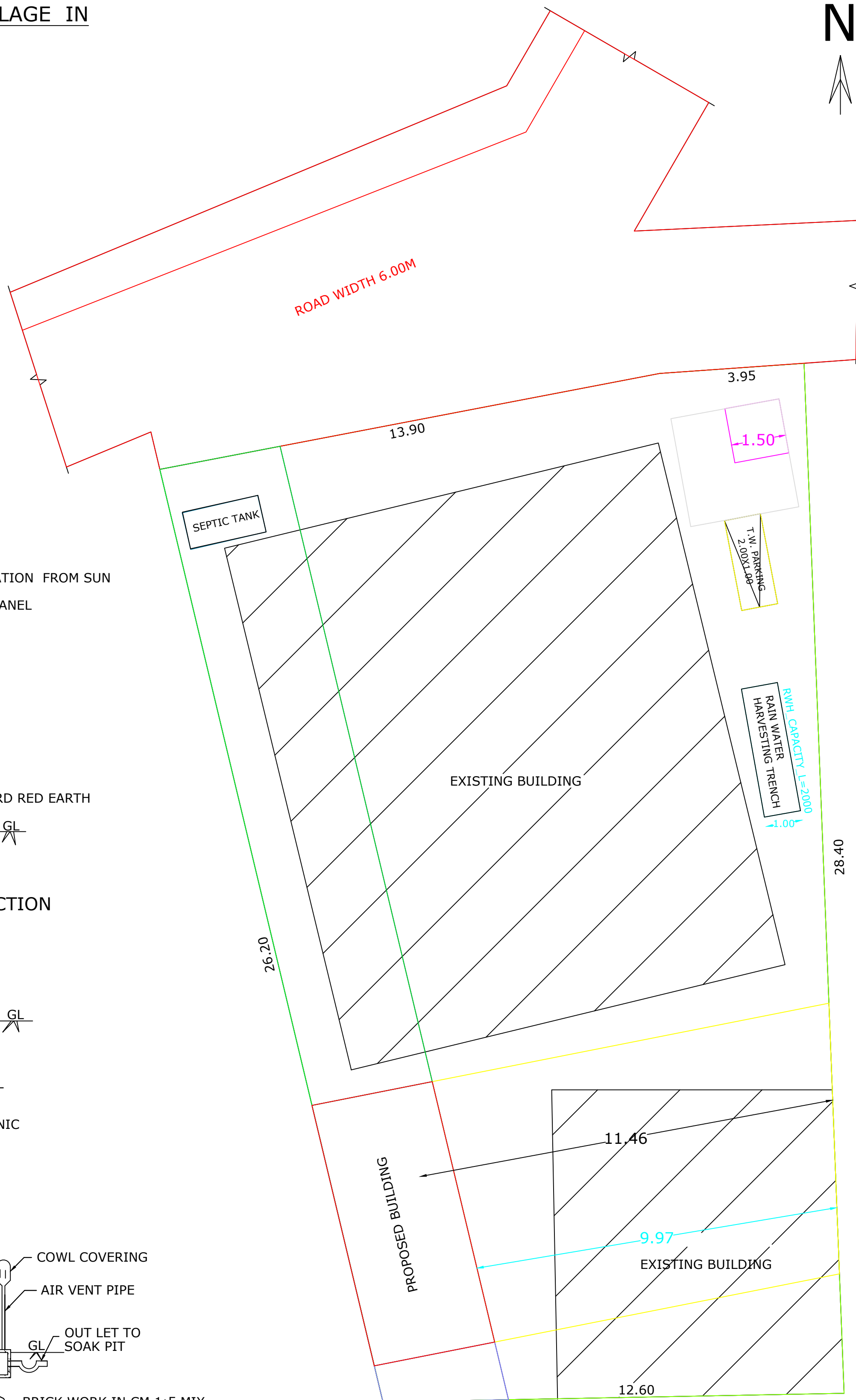
SITE PLAN
