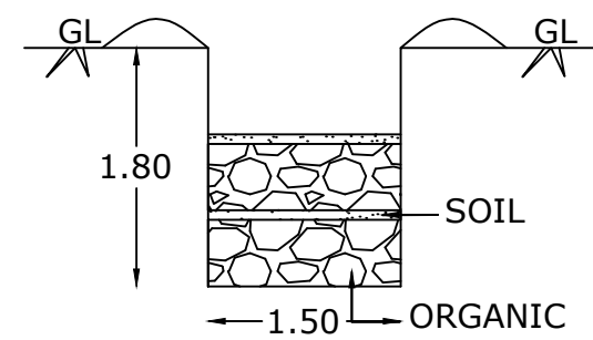
COMPOST PIT
