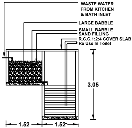
RECYCLING OF WASTE WATER FROM BATHROOM & KITCHEN
