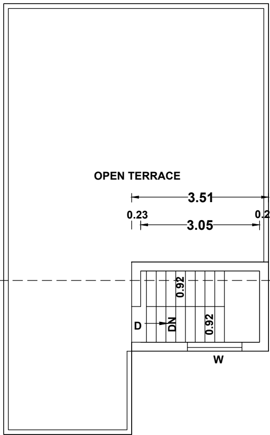
HEAD ROOM PLAN
