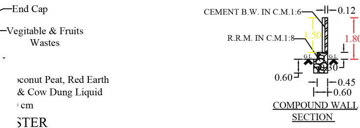
COMPOUND WALL SECTION
