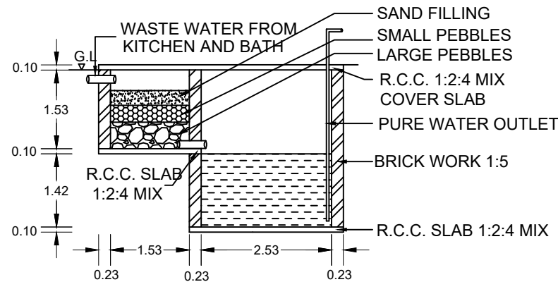
WASTE WATER RECYCLING SYSTEM
