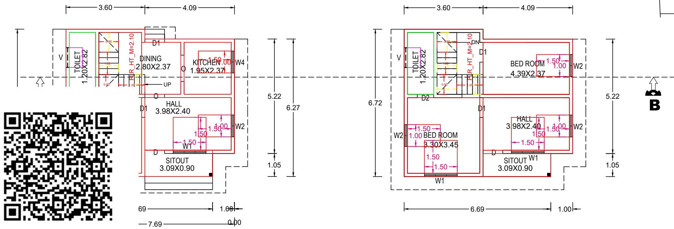
GROUND FLOOR
