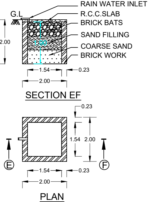
PLAN RAIN WATER PIT RWTH_CAPACITY L=5000LTRS
