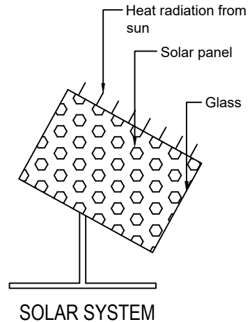
SOLAR SYSTEM
