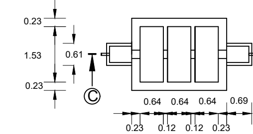
DETAILS OF SEPTIC TANK
