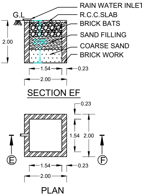
RAIN WATER PIT
