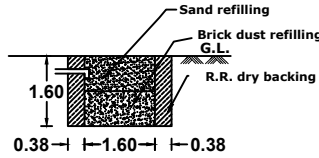
DETAILS OF RAIN WATER HARVESTING
