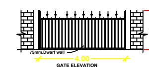
4.00 GATE ELEVATION
