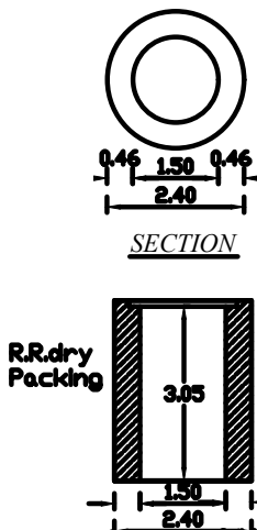
RAIN WATER HARVESTING ARRANGEMENT NOT TO SCALE
