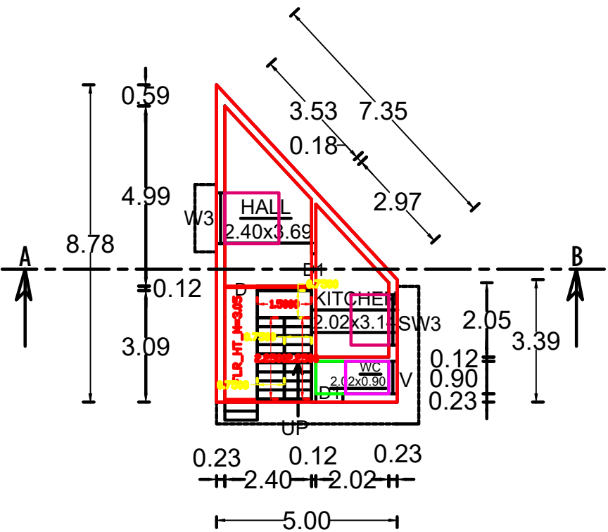
GROUND FLOOR PLAN SCALE : 1: 100 1-2.02-1
