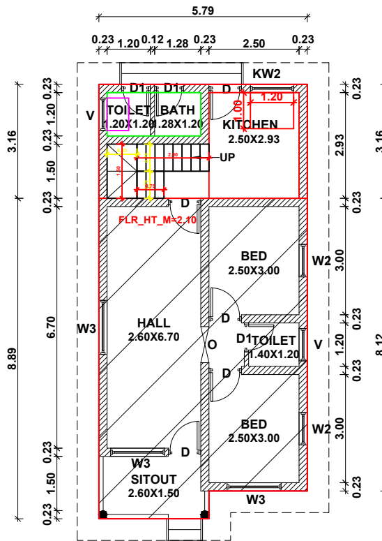
GROUND FLOOR PLAN (EXISTING & EXTENSION) BUILDING DOOR NO:2/59/1
