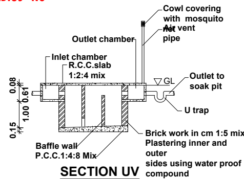
SECTION UV
