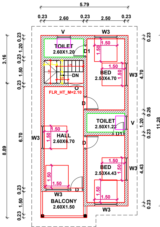
FIRST FLOOR PLAN (EXTENSION)
