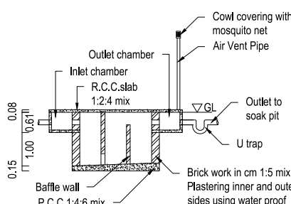
SECTION UV
