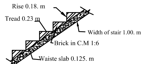
Stair Details
