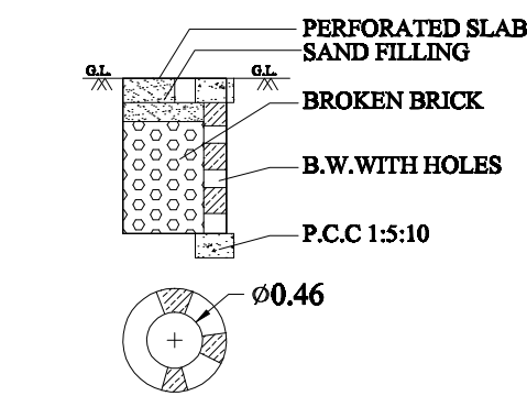
RAIN WATER PERCOLATION DRAWING TYPE -1A
