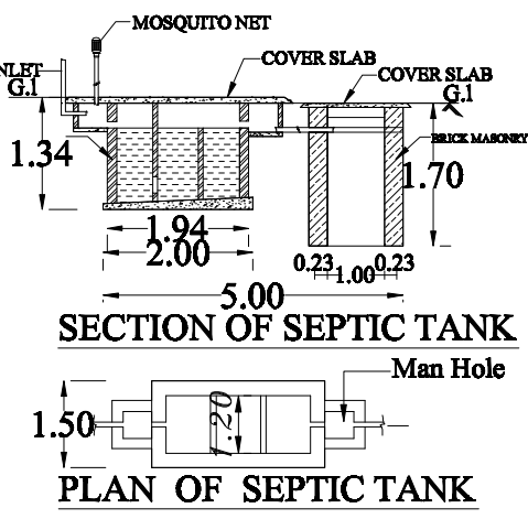
SECTION OF SEPTIC TANK PLAN OF SEPTIC TANK
