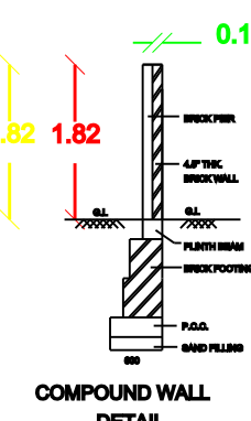
COMPOUND WALL DETAIL
