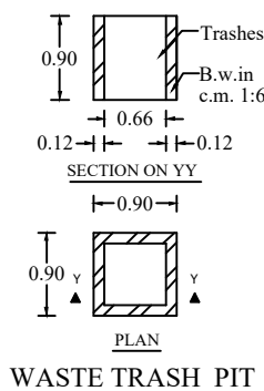
WASTE TRASH PIT
