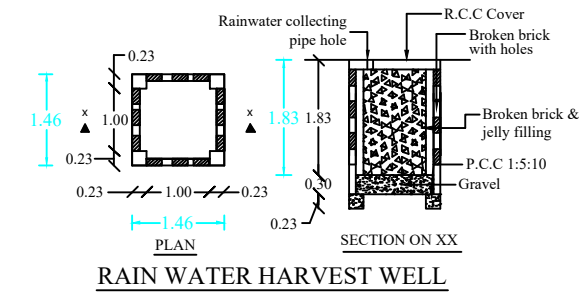
RAIN WATER HARVEST WELL PLAN RWH CAPACITY 1-6642LTRS
