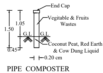
PIPE COMPOSTER
