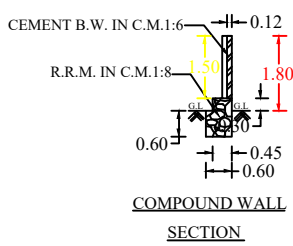
COMPOUND WALL SECTION
