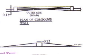
PLAN OF COMPOUND WALL
