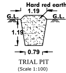
TRIAL PIT (Scale 1:100)
