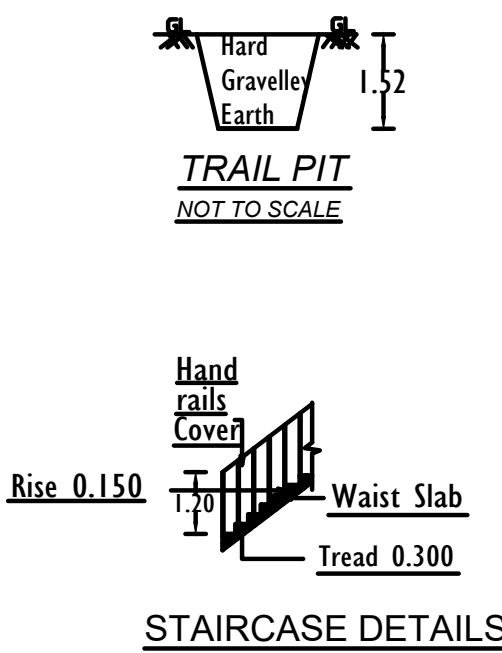
STAIRCASE DETAILS
