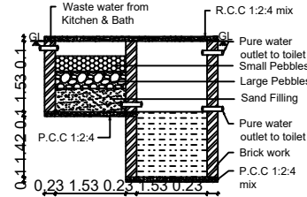
WASTE WATER RECYCLING PIT
