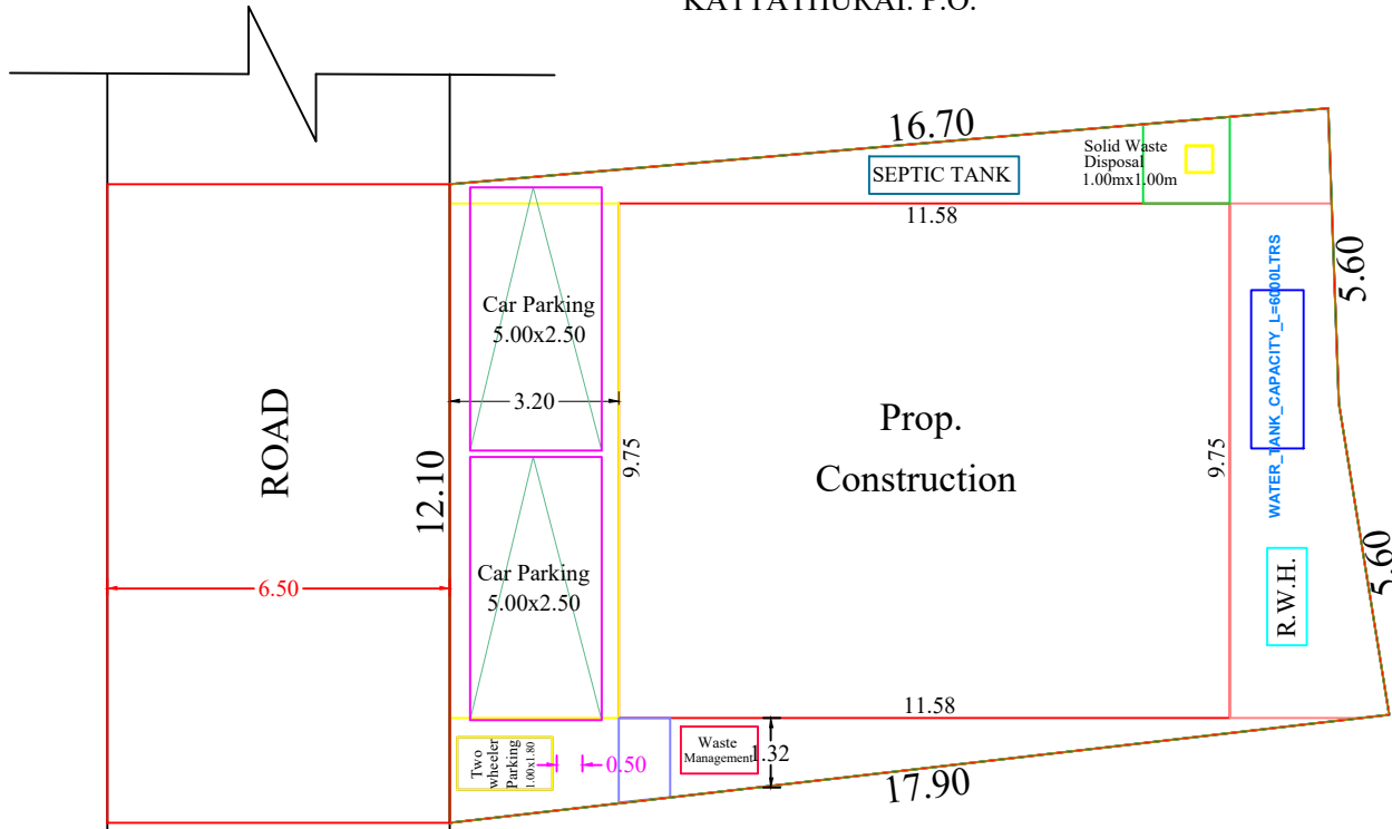
SITE PLAN
