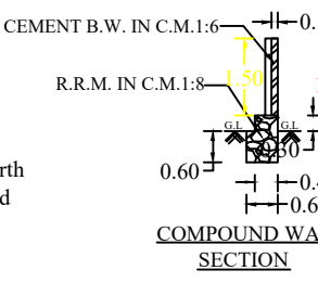
COMPOUND WALL SECTION
