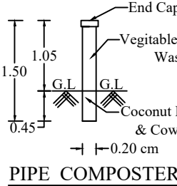
PIPE COMPOSTER
