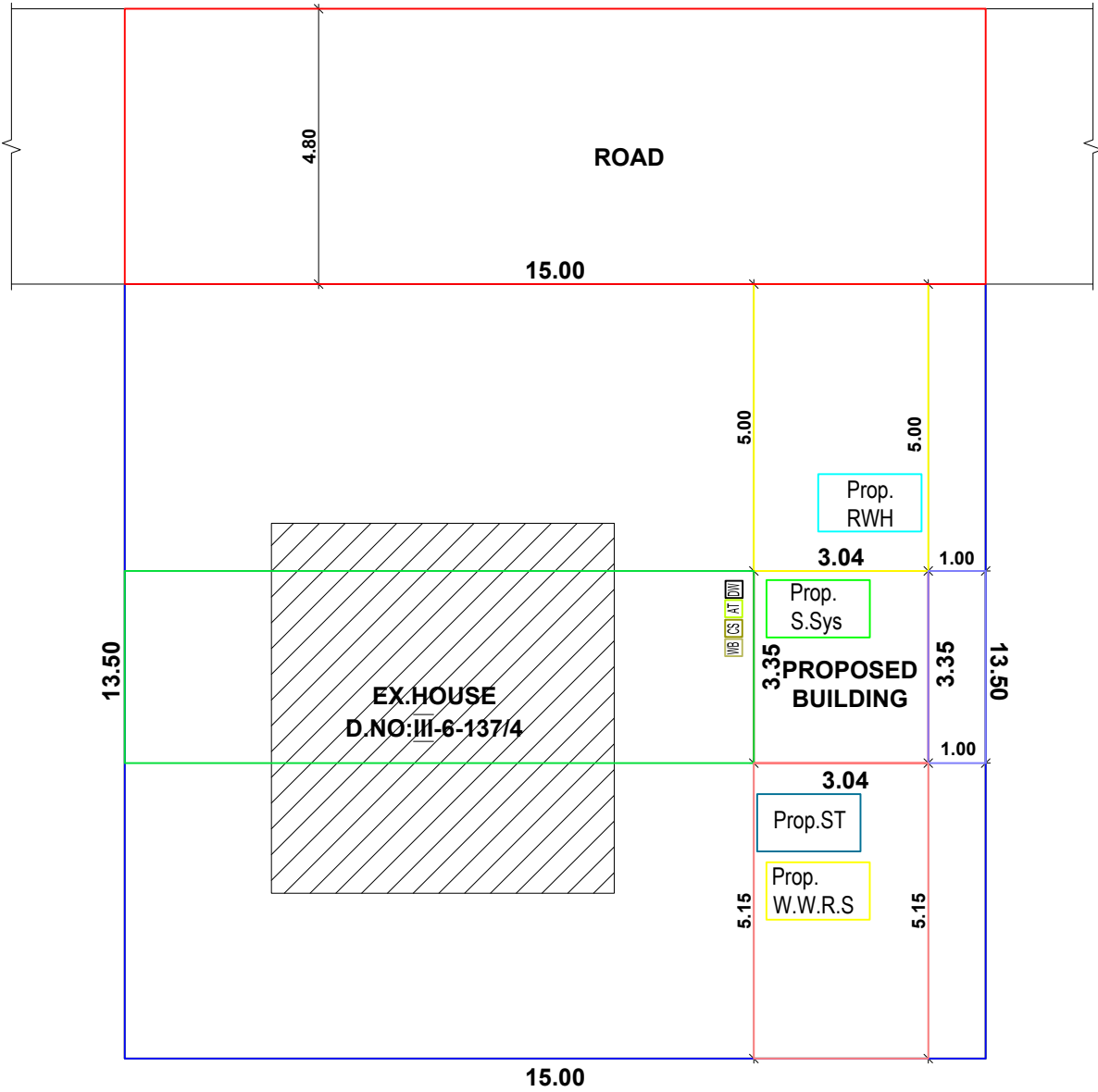
SITE PLAN
