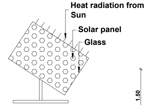
SOLAR SYSTEM
