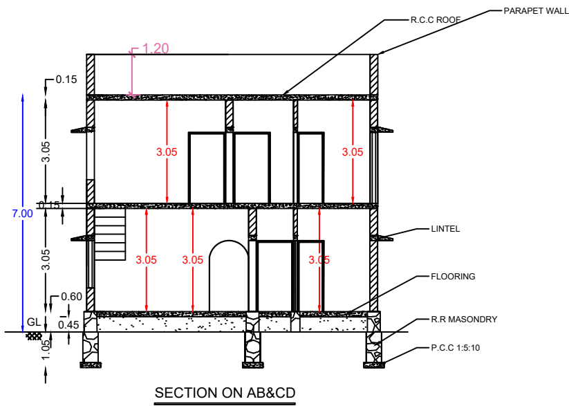
SECTION ON AB&CD
