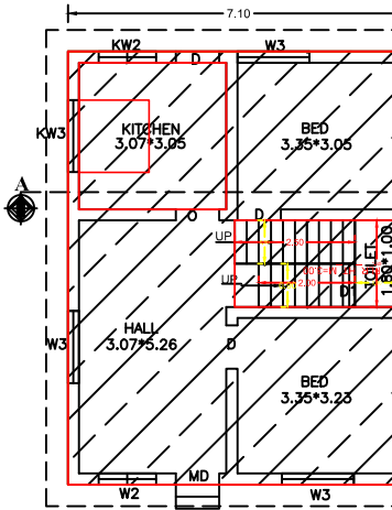
EX.GROUND FLOOR PLAN
