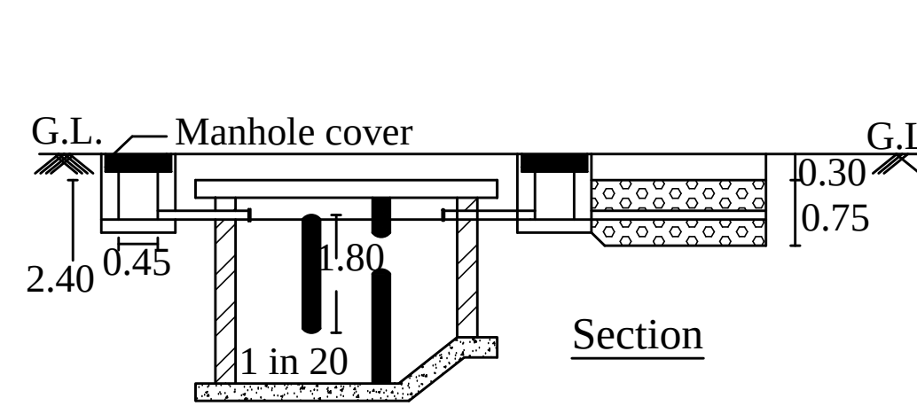
Rain Water Storage
