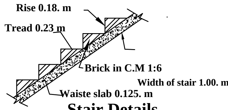
Stair Details
