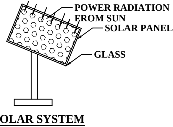
SOLAR SYSTEM
