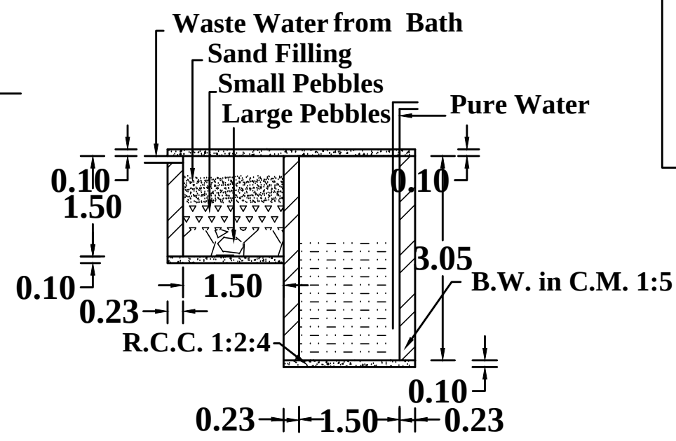
WASTE WATER RECYCLING SYSTEM
