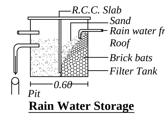
Rain Water Storage
