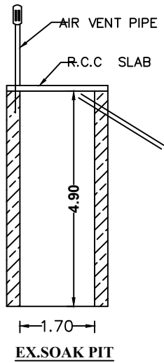
EX-SOAK PIT
