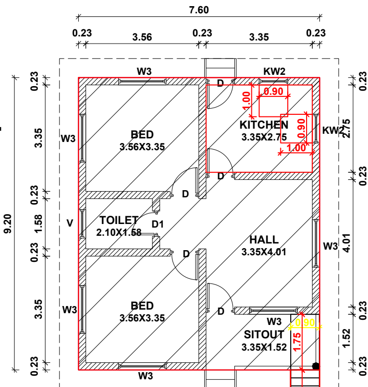
EX.GROUND FLOOR PLAN
