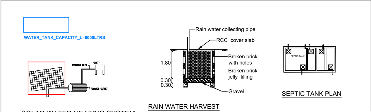
RAIN WATER HARVEST WELL SECTION
