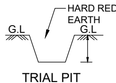
TRIAL PIT
