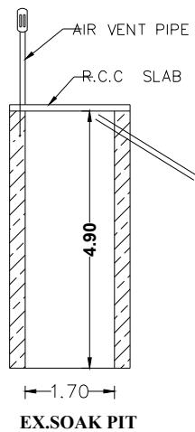
EX-SOAK PIT
