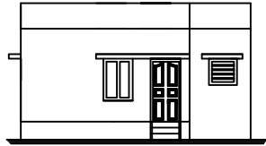
FRONT ELEVATION
