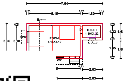
FLOOR PLAN
