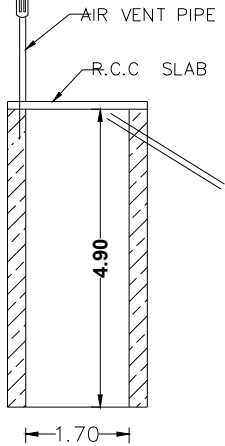
EX-SOAK PIT
