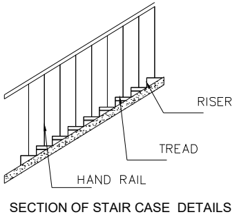
SECTION OF STAIR CASE DETAILS
