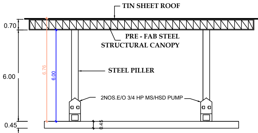
SECTION ON A1-B1
