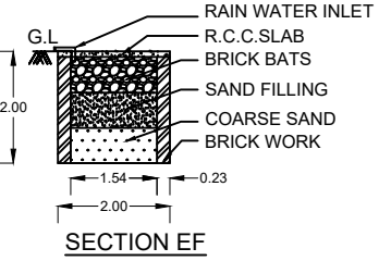
SECTION EF
