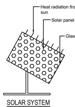
SOLAR SYSTEM
