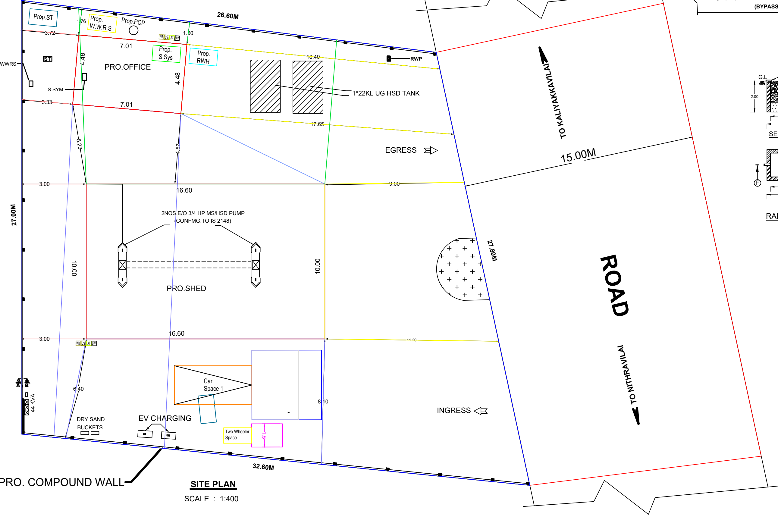
PLAN
