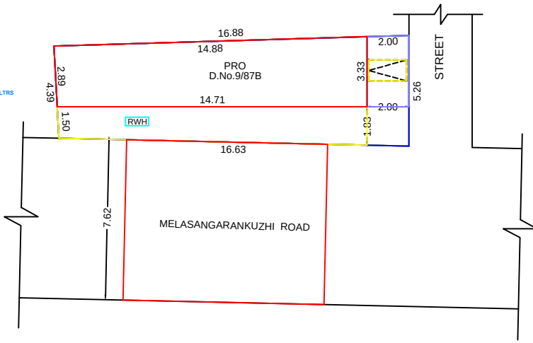
SITE PLAN
