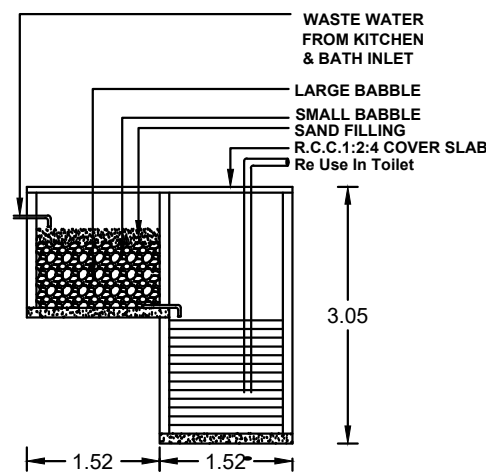
RECYCLING OF WASTE WATER FROM BATHROOM & KITCHEN
