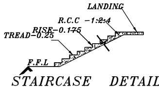
STAIRCASE DETAIL
