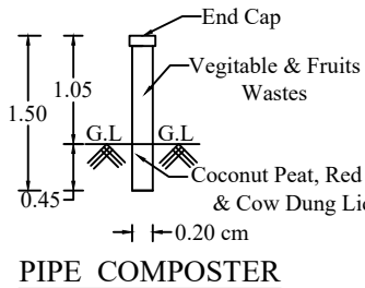
PIPE COMPOSTER
