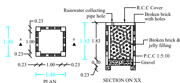
RAIN WATER HARVEST WELL
