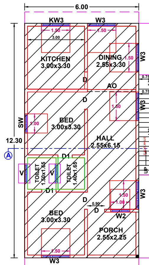
GROUND FLOOR PLAN PORTION-1
