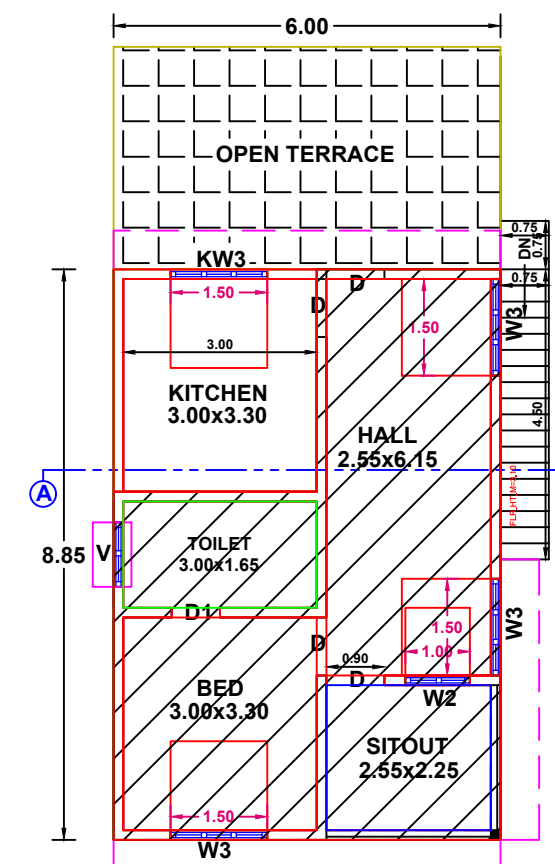
FIRST FLOOR PLAN PORTION-2
