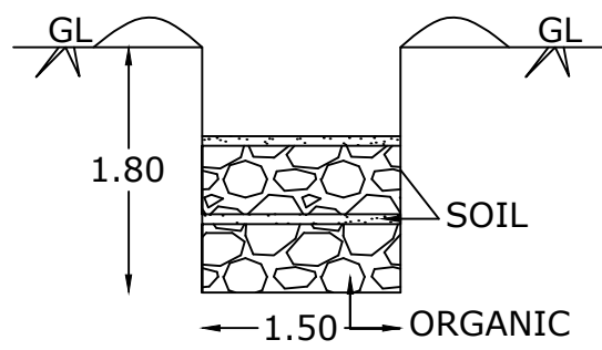
COMPOST PIT
