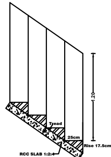
STAIR DETAILS
