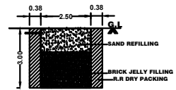
DETAILS OF RAIN WATER HARVESTING
