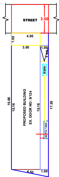
SITE PLAN
