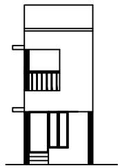
FRONT ELEVATION
