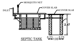
SEPTIC TANK
