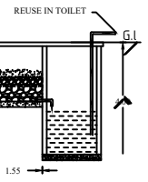
RAIN WATER INLET TYPE - 1 A
