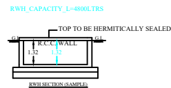
RAIN WATER INLET TYPE - 1 A
